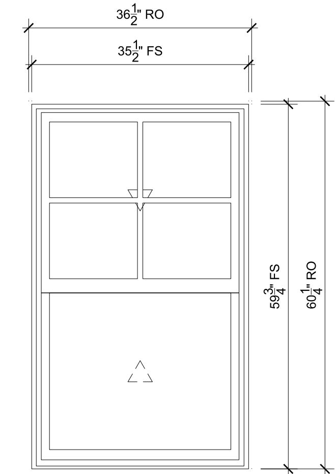
LEFT - FAMILY ROOM SCALE: 3/4" = 1'-0"
