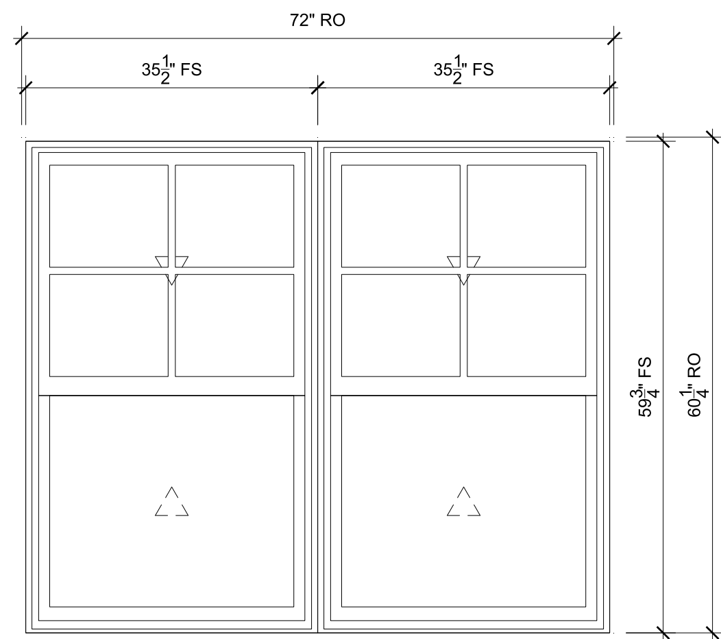
FRONT - STUDY SCALE: 3/4" = 1'-0"
