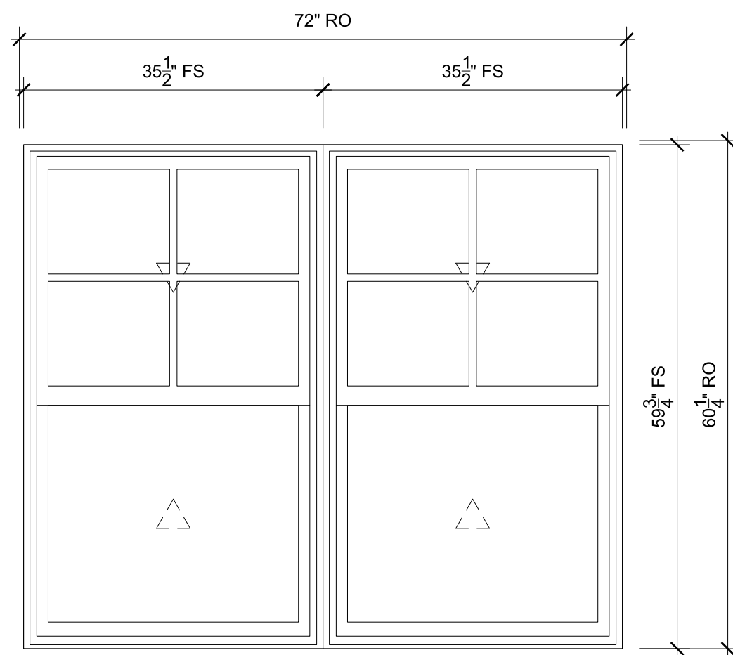
FRONT - DINING SCALE: 3/4" = 1'-0"
