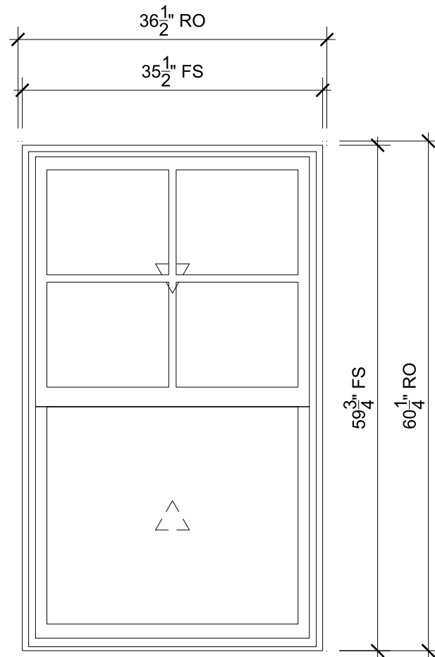
FRONT - GARAGE SCALE: 3/4" = 1'-0"
