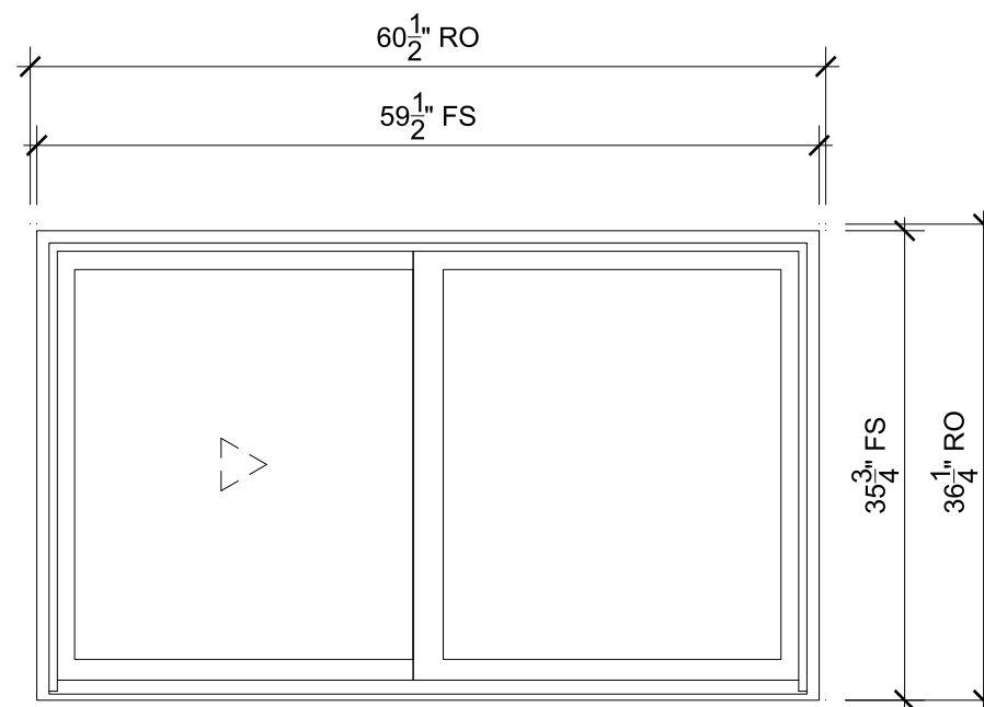
BASEMENT EGRESS SCALE: 3/4" = 1'-0"
