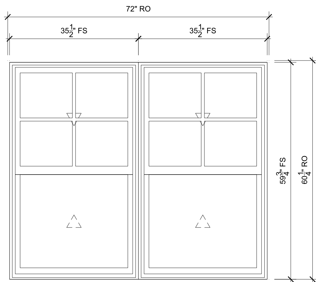
FRONT - MASTER SCALE: 3/4" = 1'-0"
