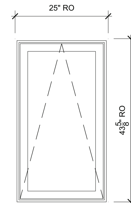
NORTH N SCALE: 3/4" = 1'-0"
