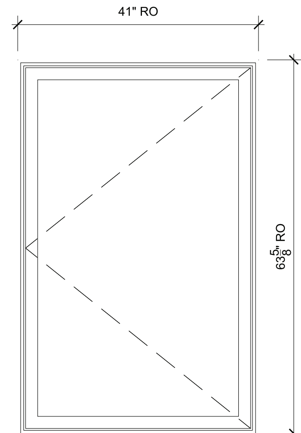
EAST X SCALE: 3/4" = 1'-0"
