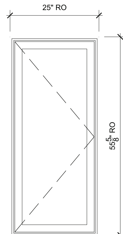
NORTH L SCALE: 3/4" = 1'-0"
