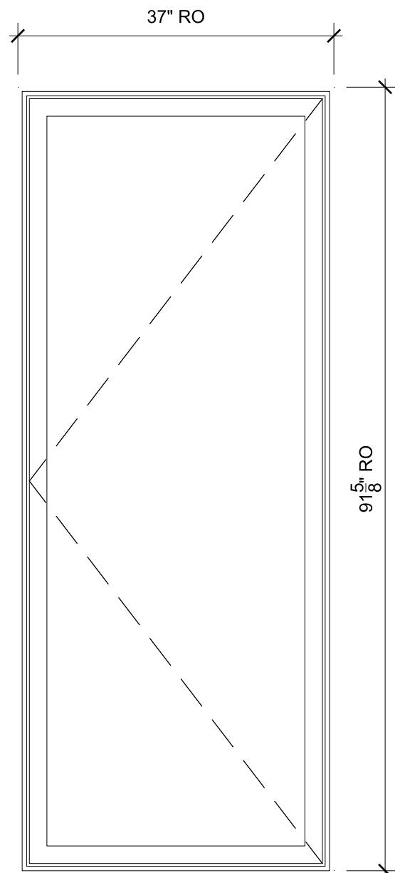
EAST V SCALE: 3/4" = 1'-0"
