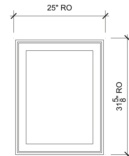
NORTH M SCALE: 3/4" = 1'-0"
