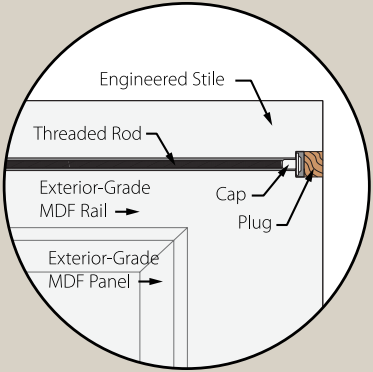
All exterior MDF doors come with our exclusive TruBolt system for added strength
