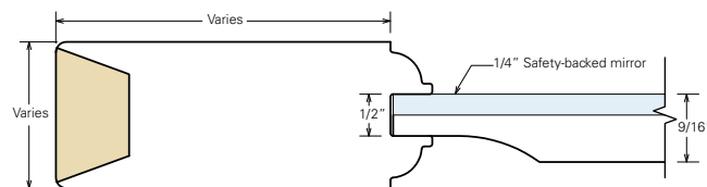
Sample cross section (one-sided mirror door)
