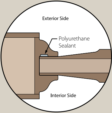
The Sentry Protective System provides a weatherproof seal around all panels and glass
